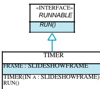
FIGURE 15.11 The Timer class delays the frame thread between each
