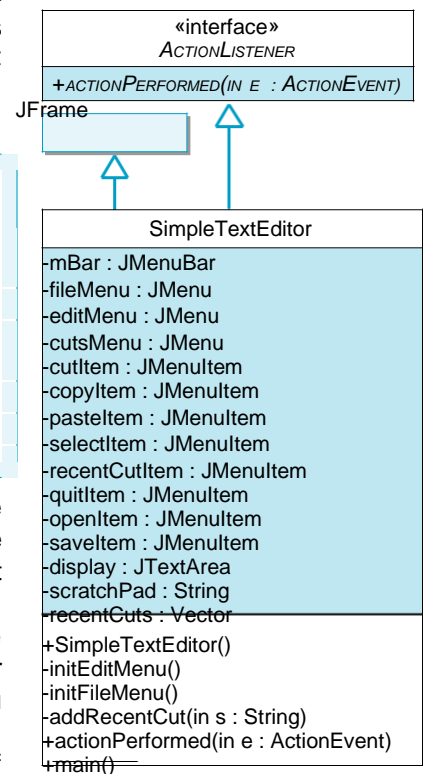
Figure 13.32: Design of the SimpleTextEditor .
