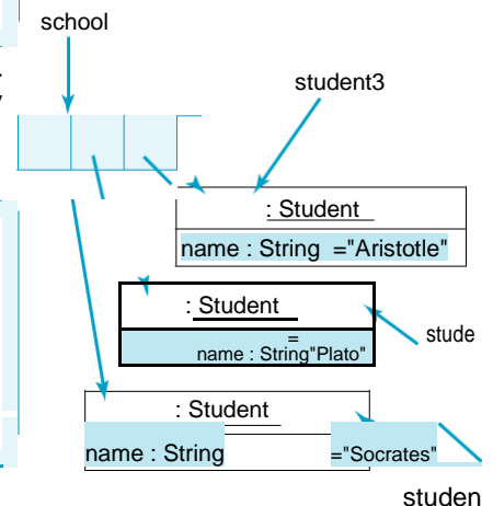
Figure 9.4: Arrays of objects store references to the objects, not the objects themselves.
