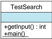
Figure 9.17: The TestSearch class.
