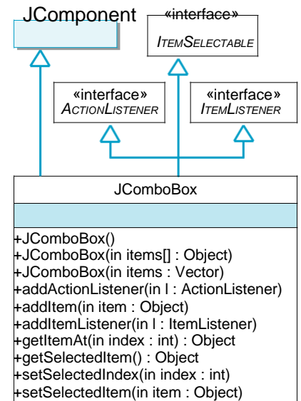
Figure 12.28: A JComboBox responds to action events and item events.
