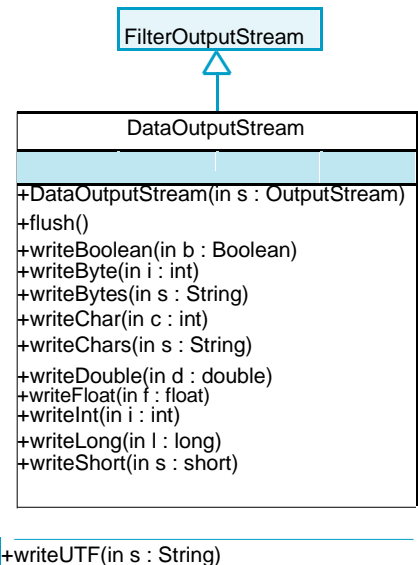
Figure 11.18: The java.io.DataOutputStream class contains methods for writing all types of data.
