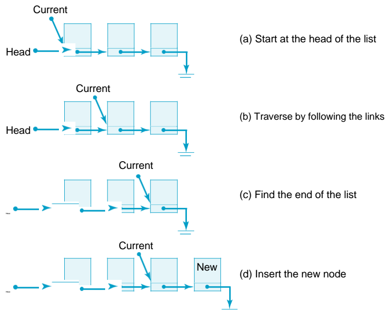
Figure 16.9: The temporary variable current is used to traverse the list to find its end.
