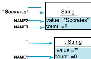
Figure 7.4: The variables name1, name2, and name3 serve as references to the literal String objects "Socrates" and "".
