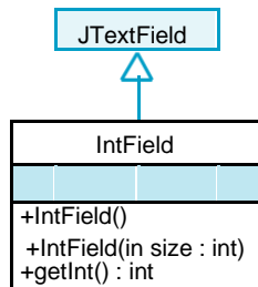
Figure 10.13: An IntField is a JTextField that accepts only integers.
