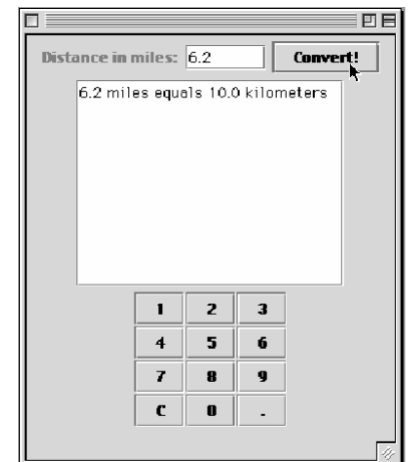
Figure 13.21: This version of the metric converter GUI uses a keypad for mouse-based input. It has an attractive overall layout.
