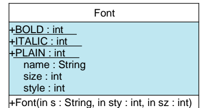
Figure 7.19: The Font class.
