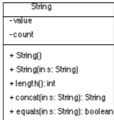
Figure 2.1: A partial representation of the String class.
