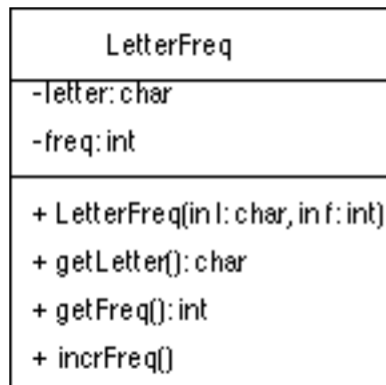
Figure 9.9: UML for 9.4.2 A Class to Count Letter Frequencies LetterFreq.
