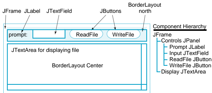
Figure 11.5: The GUI design for a program that reads and writes text files.
