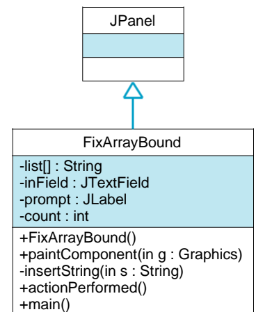
Figure 10.17: The FixArrayBound class uses exception handling to
