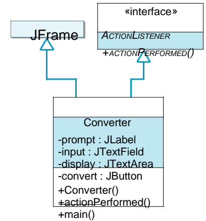
Figure 13.11: The Converter class is a subclass of JFrame and implements the ActionListener interface.
