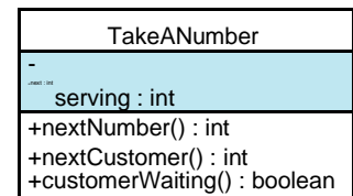
Figure 14.25: The revised TakeANumber class.
