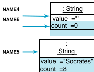
Figure 7.5: Together with the objects in Figure 7.4, there are now four different String objects with eight different references to them, including the literals "Socrates" and "".
