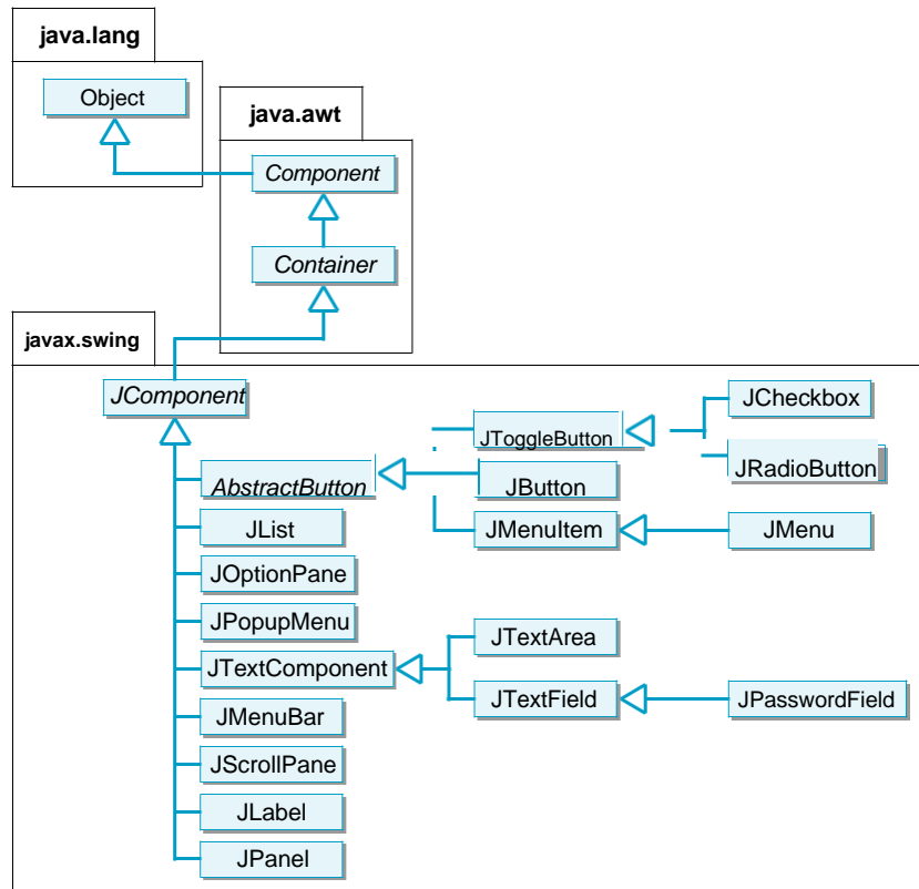
Figure 13.2: Swing classes, part Swing GUI components are derived from the JComponent class.
