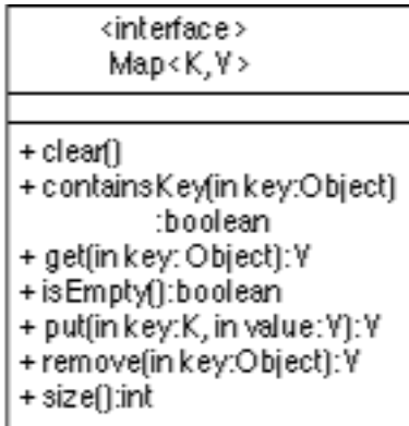
Figure 16.34: A partial list of methods of Map<K,V>.
