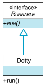
Figure 14.14: In a multithreaded design, the Dotty class implements Runnable.
