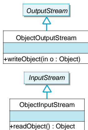
Figure 11.26: Classes used for performing I/O on objects.
