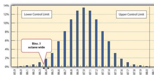
Figure 14.1 Normal Distribution of Measurements
