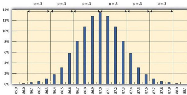
Figure 14.3 The 68-95-99.7 Rule
