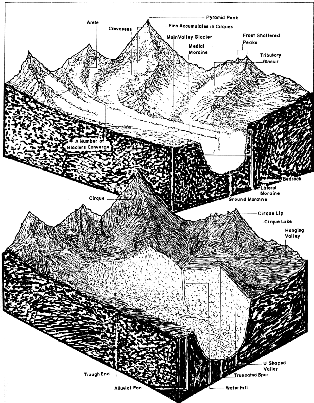
Figure 4.18: Glaciated landscape
