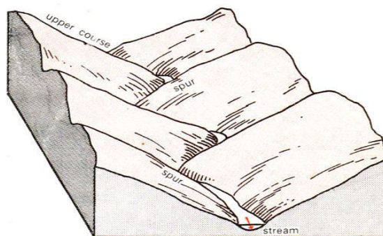
Figure 4.28: Interlocking Spurs
