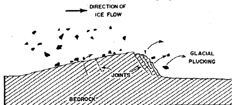
Figure 4.14: Roche moutonnee
